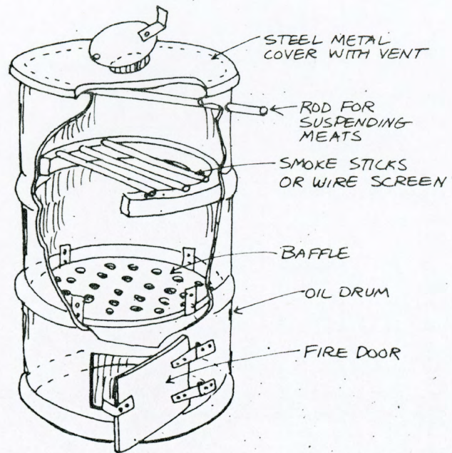
A smoker made from a metal 55-gallon drum. (Originally published in UGA Extension Bulletin 865, "Sausage and Smoked Meats.")
