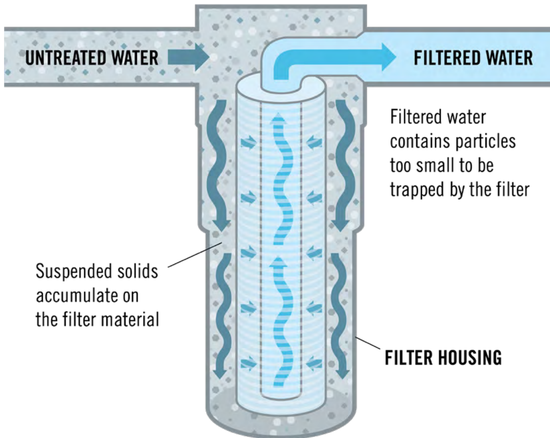
Figure 1. The sediment filtration process.
