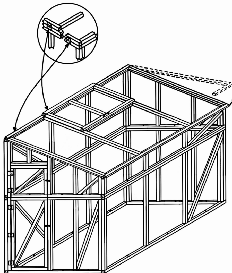
Greenhouse Assembly
