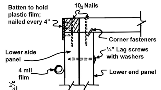
FASTENING DETAIL
